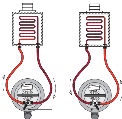
fig. 1 - Clockwise circulation
